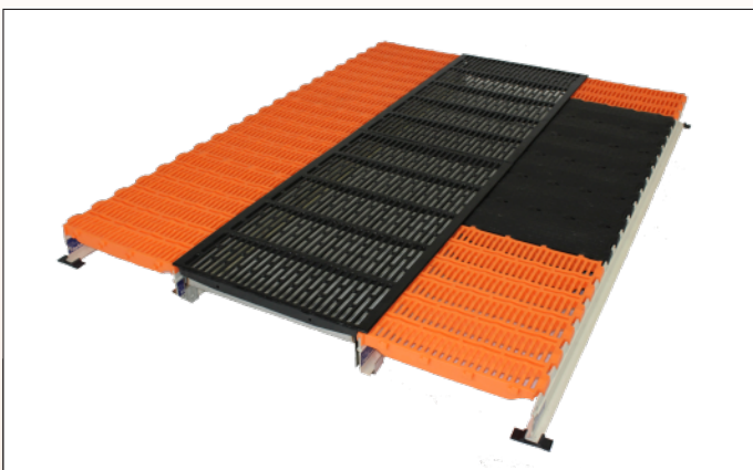
The Farmweld Warming Panel™ reduces drafts to keep newborn piglets warm , and the panel texture offers superior traction. Made with virgin polypropylene material, the interlocking design integrates seamlessly into the Farmweld cast platform, beams and flooring system. Sizes allow producers flexibility in determining coverage area.
